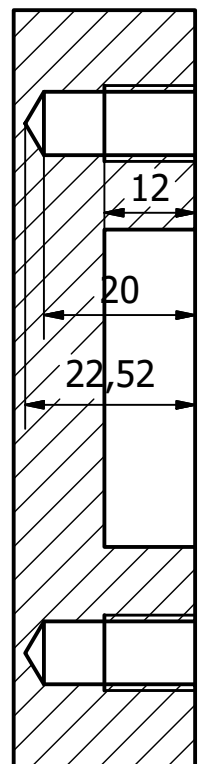
C-C ( 1 )
