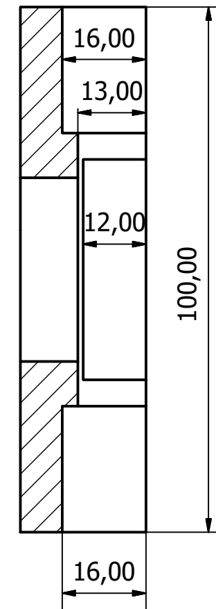
B-B ( 1 )
